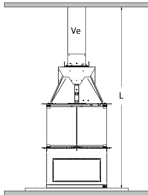
Figure 10: Clearances - Ceiling
