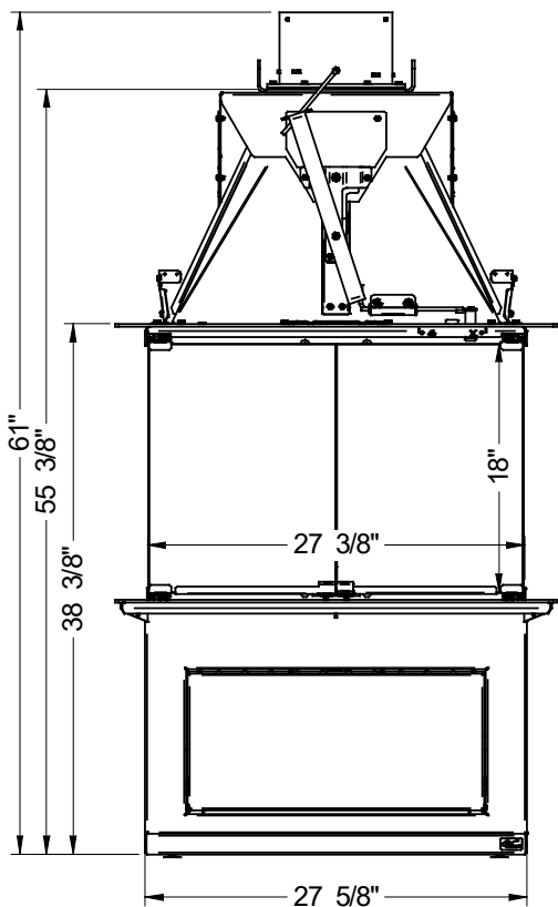
Figure 2: Front View
