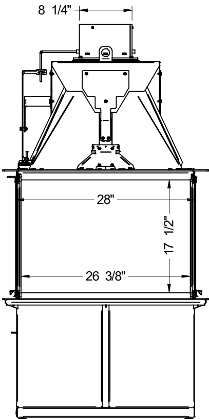
Figure 3: Side View
