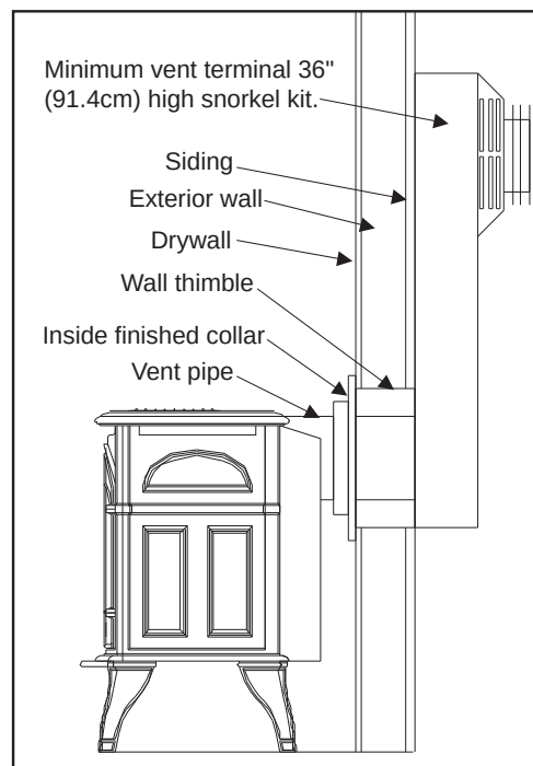
Figure 42: Installation for Rear Vented; 30,000 Btu/hr.
