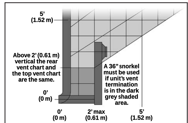
Figure 24. Possible Vent Configurations for Rear Vented; Vertical and Horizontal Terminations.
