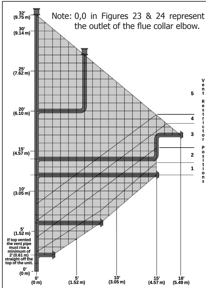
Figure 23. Possible Vent Configurations for Top Vented; Vertical and Horizontal Terminations.
