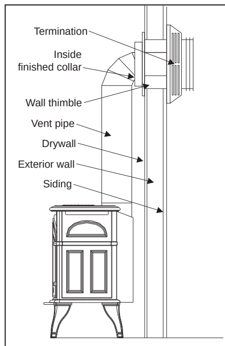
Figure 43: Installation for Top Vented; Horizontal Termination.
