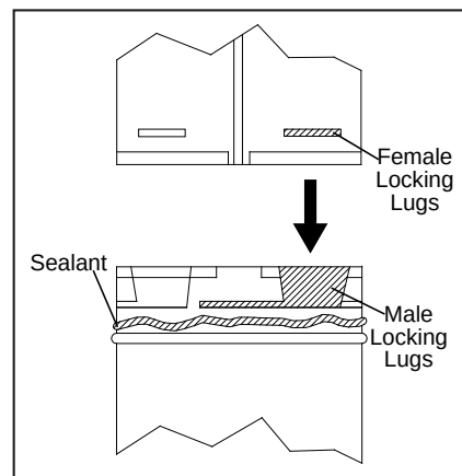
Figure 25: Twist-Lock Connection
