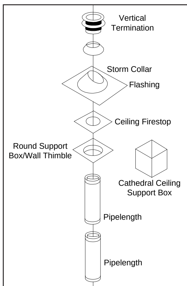
Figure 16: Common Vertical Installation.
