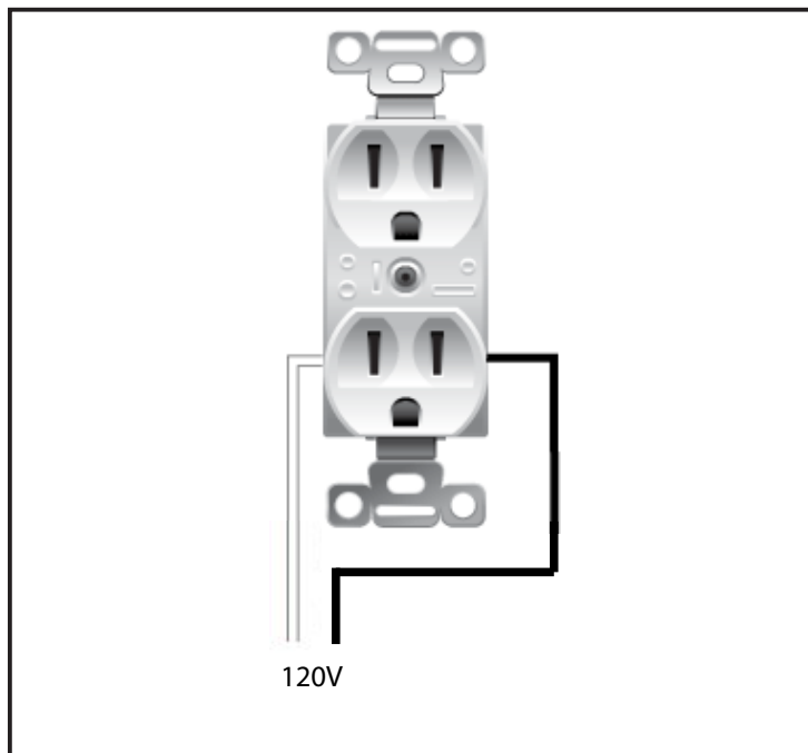
Figure 52: C72I Receptacle Wiring
