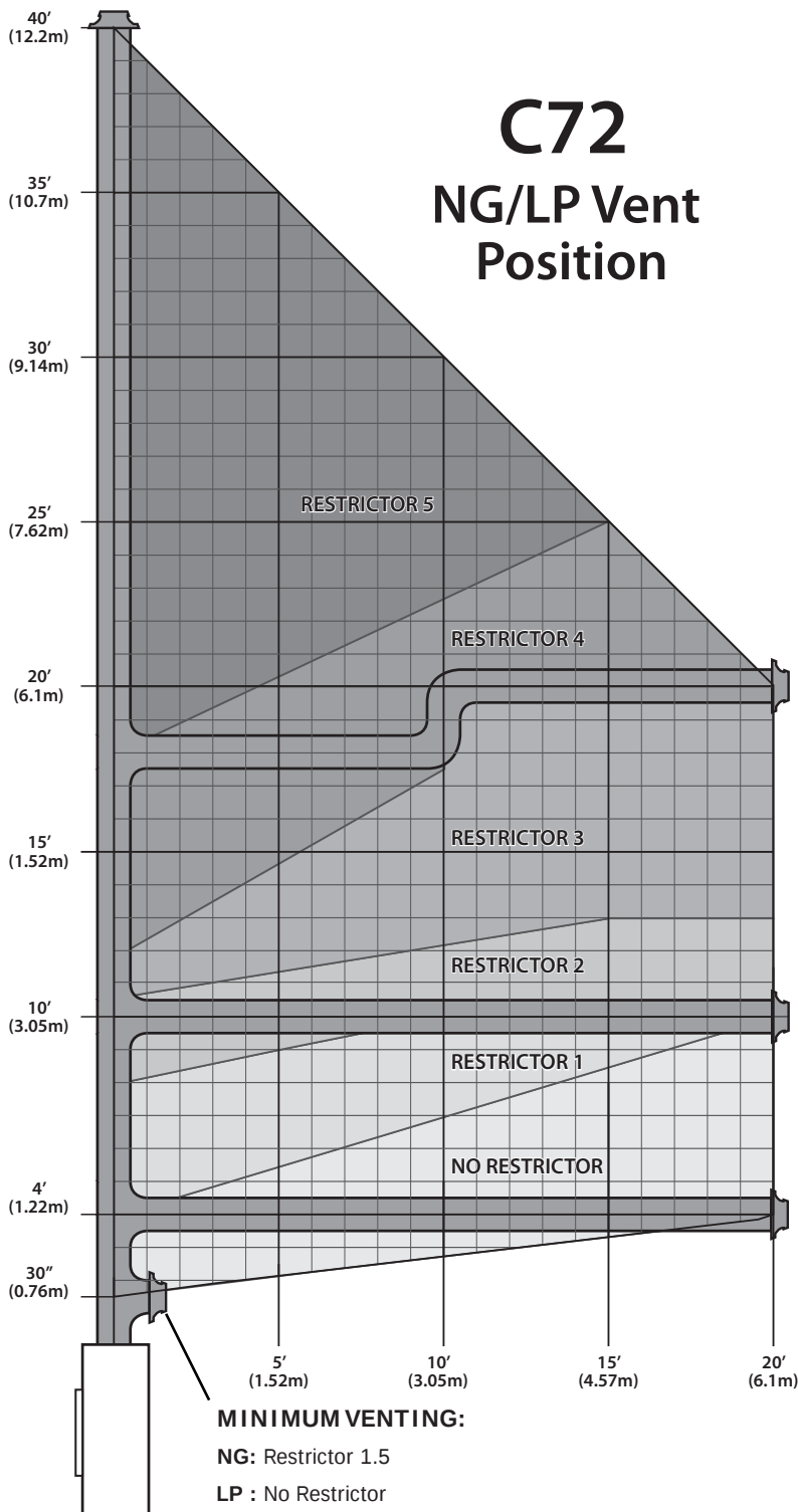
Figure 42. NG/LP Vent Graph
