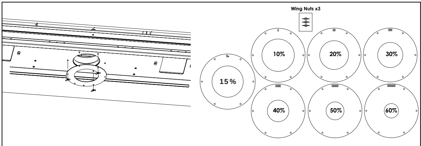
Figure 43. Restrictor Install and Ring Set
