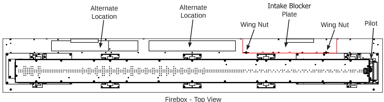
Figure 44. Intake Blocker Plate
