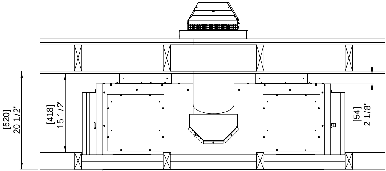
Figure 35(a). Dimensions for a Horizontal Installation
