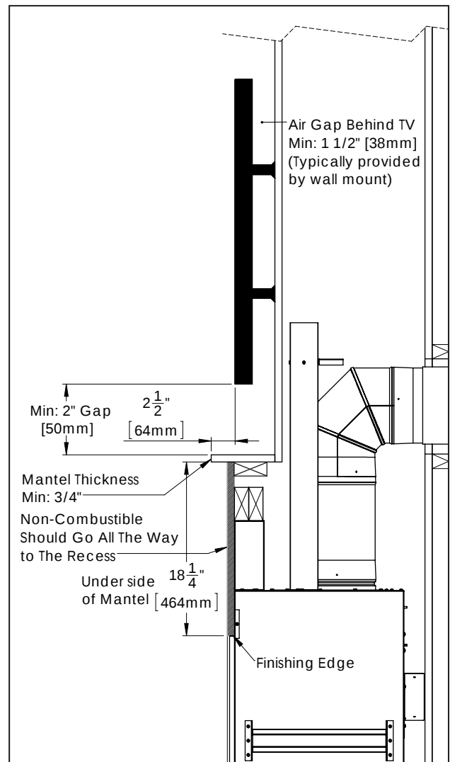
Figure 39. Recess Minimum TV Install Clearances
