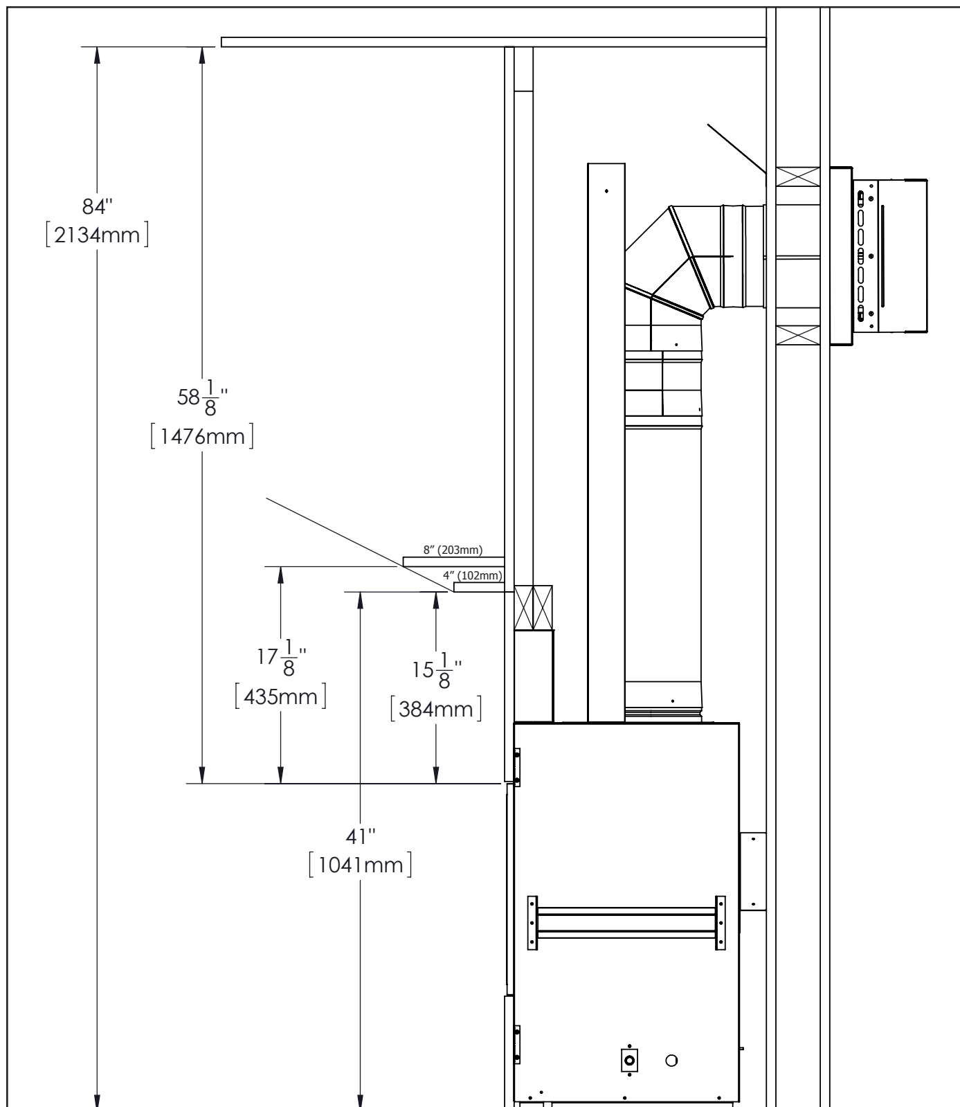
Figure 30(b): Install Dimensions with Mantel
