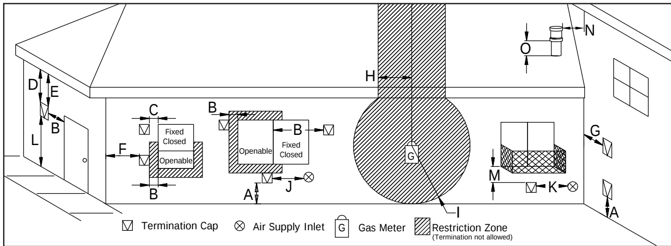
Figure 40. Vent Termination Restrictions, refer to Table 2
