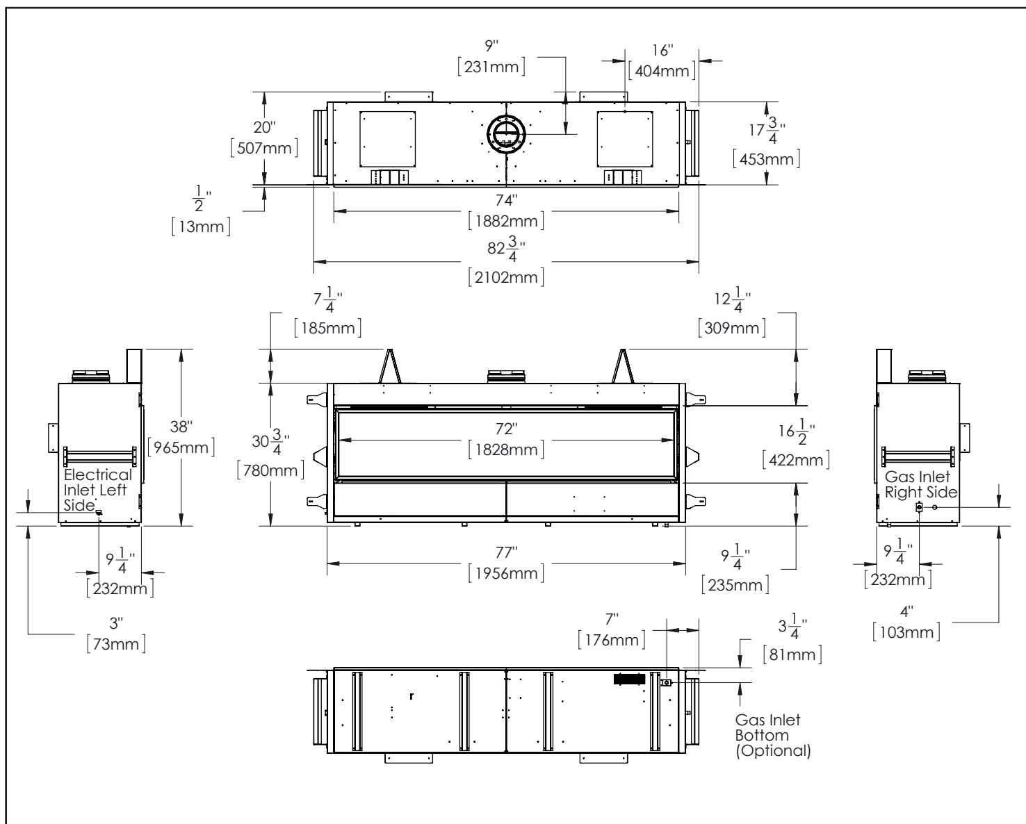
Figure 1. Unit Dimensions
