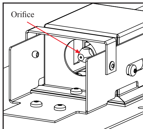
Figure 23: Orifice location
