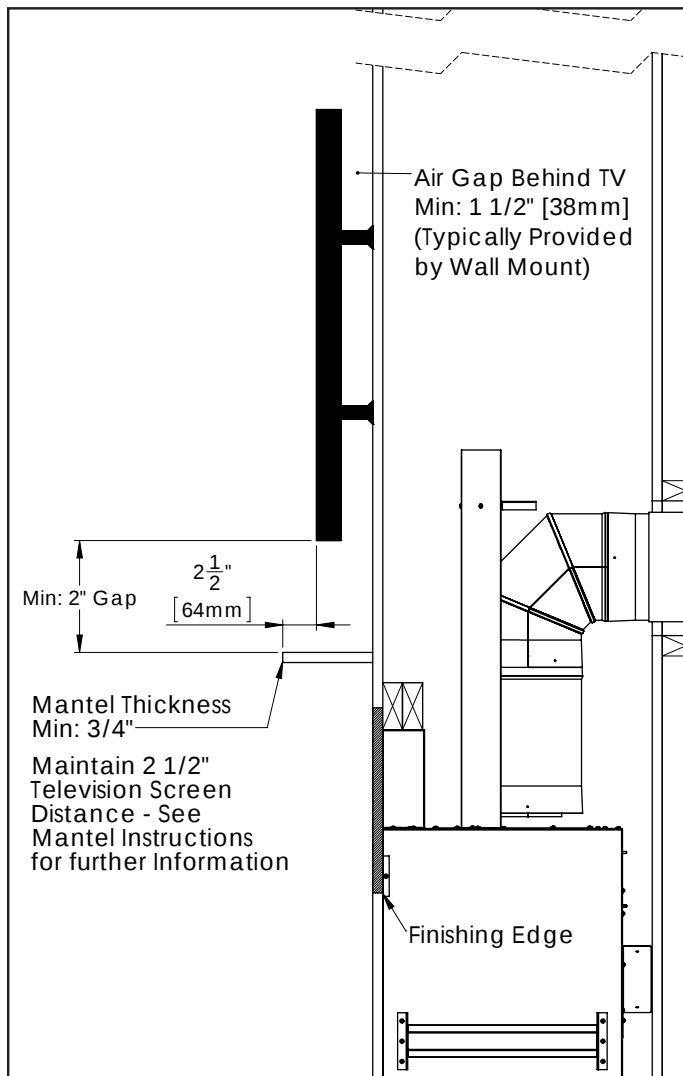
Figure 38. Minimum TV Install Clearances
