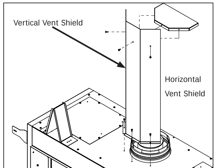
Figure 34. Vent Shielding Install
