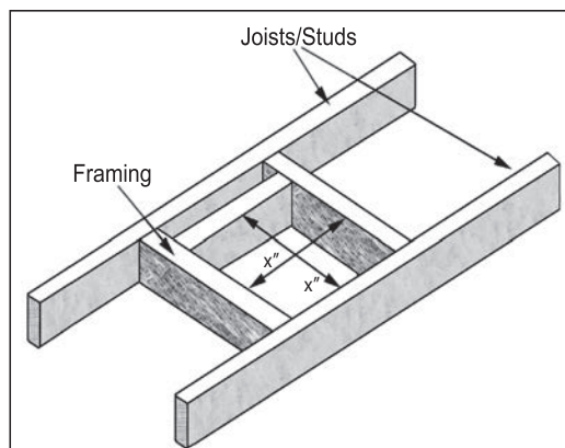
Figure 41. Vent Framing For Wall or Ceiling
