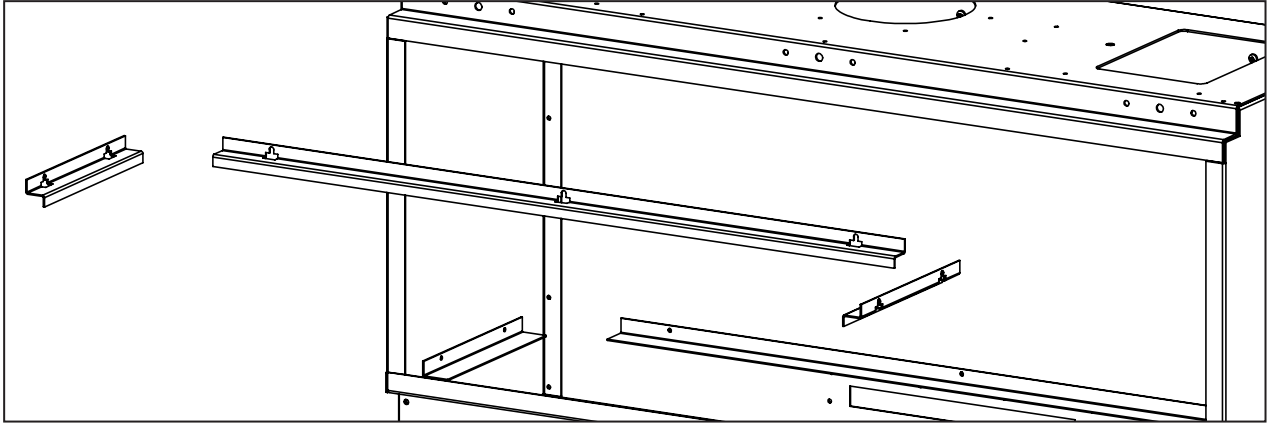
Figure 56: Panel Installation
