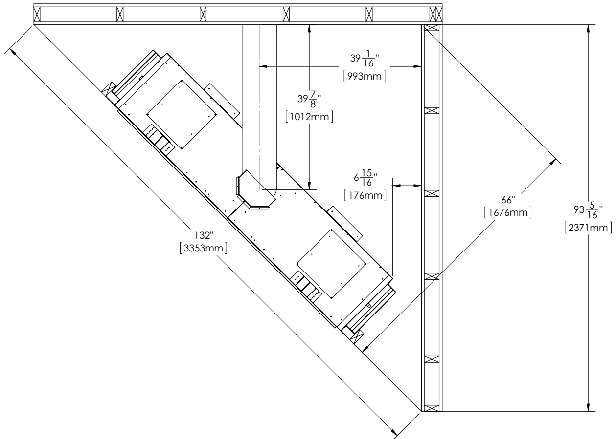
Figure 33. Dimensions for a Corner Installation
