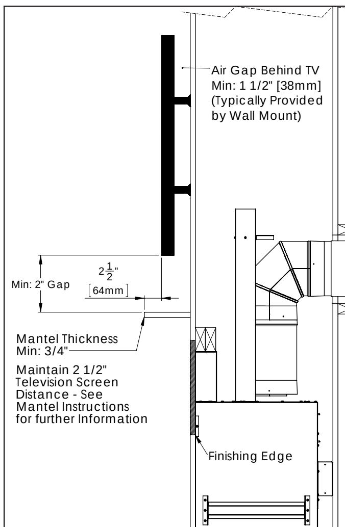
Figure 52: Minimum TV Install Clearances
