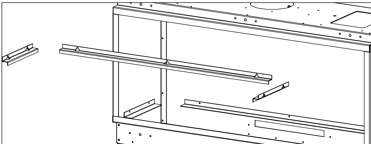
Figure 73: Panel Installation
