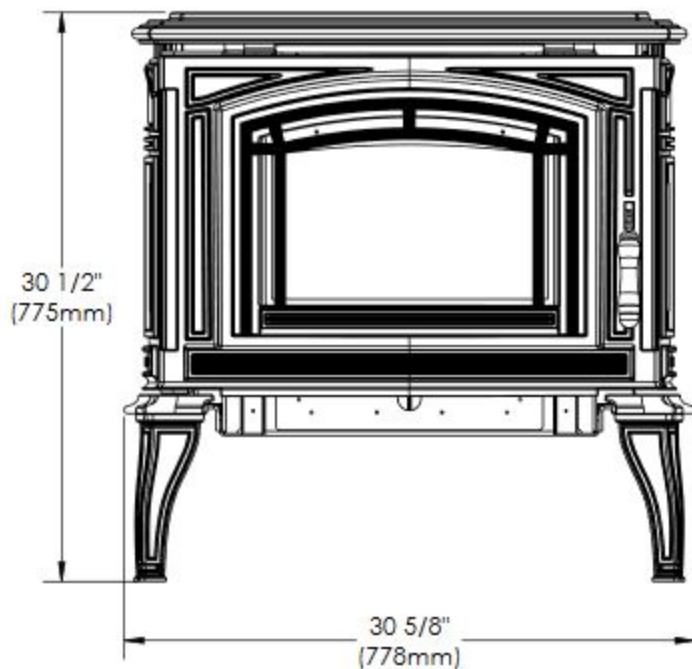
Figure 14: Meridian Cast Iron Dimensions.
